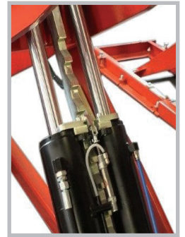
Sicurezza meccanica AT-ATLT Mechanical locking system AT-ATLT
